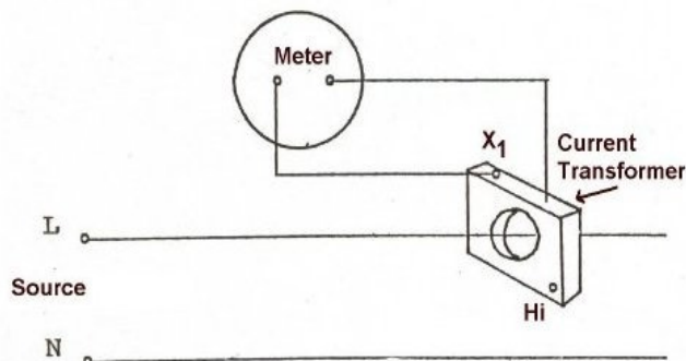
ACA Meters: 0-5 ACA CT/Transformer-rated
