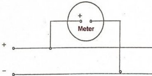
DCmV / DCV Meters
