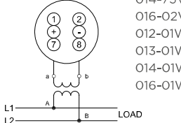
VOLTMETER AC/ FREQUENCY METER V.T. operated
