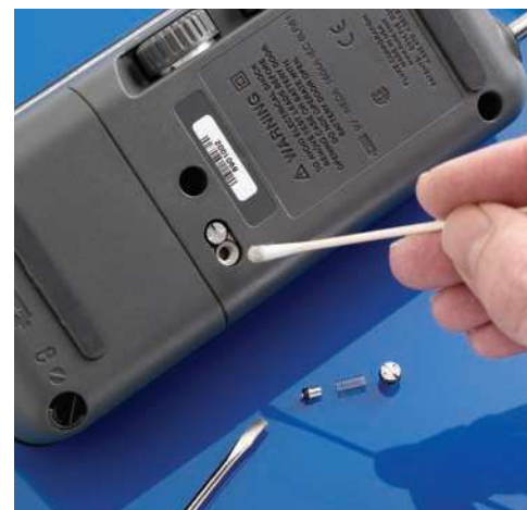
Cleaning the fluid trap in the Fluke-718 Calibrator is quick, easy and only requires a slotted screwdriver and cotton swab
