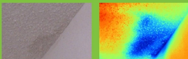
Unexpected moisture intrusion in a ceiling.
